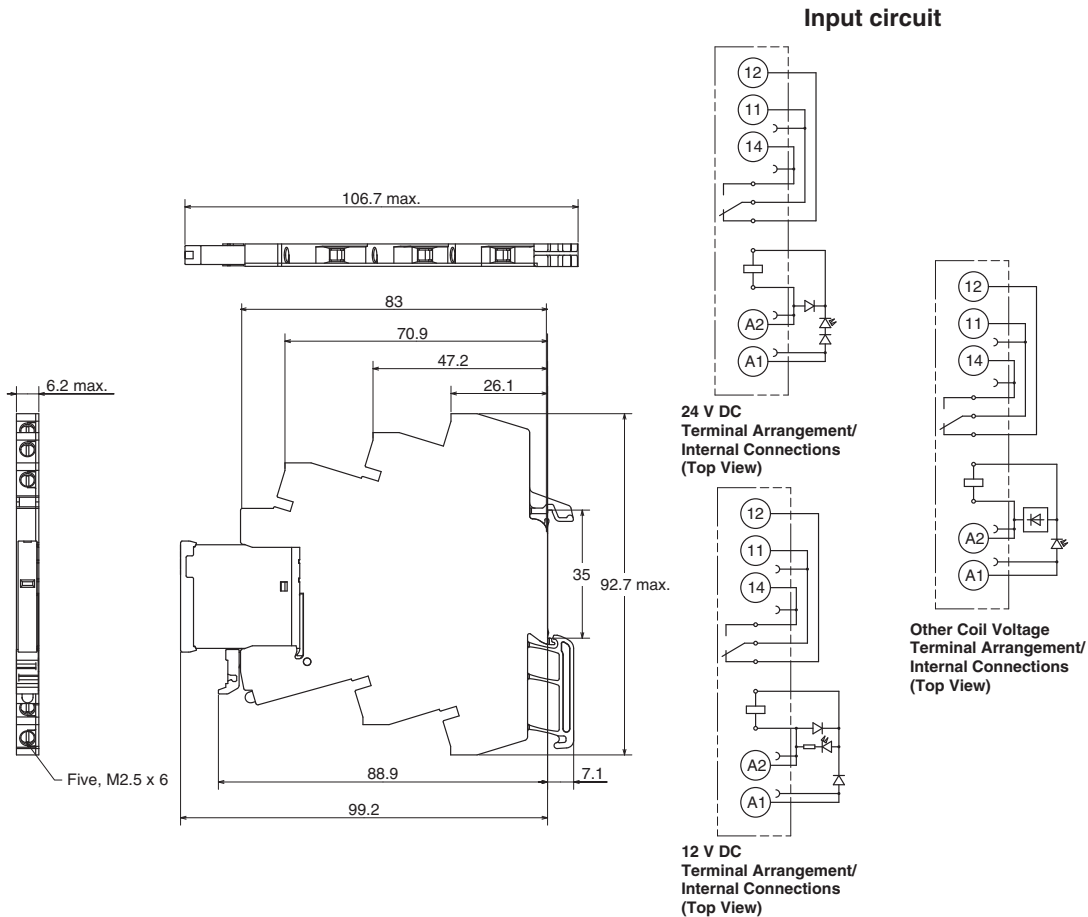
Input circuit
